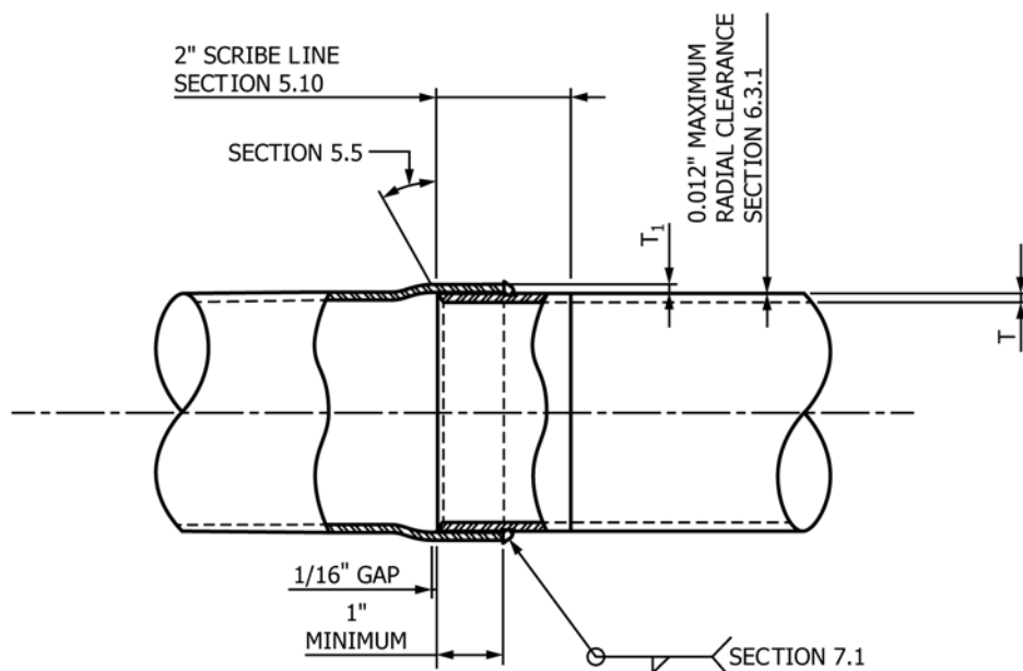
NOTE 1—1 in. = 25.4 mm. FIG. 1 Expanded Welded Socket Joint
