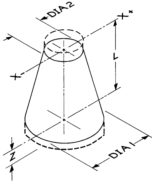
FIG. 23 Shape 5.1—Reducer-Round
