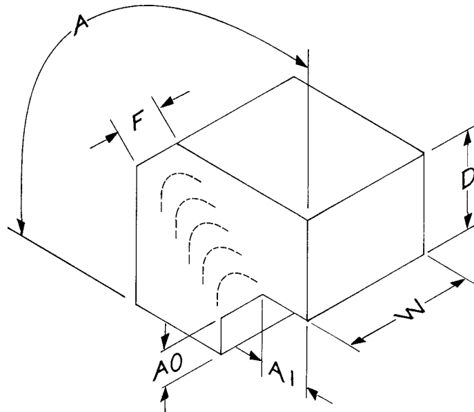
FIG. 22 Shape 4.1—Vaned Turn
