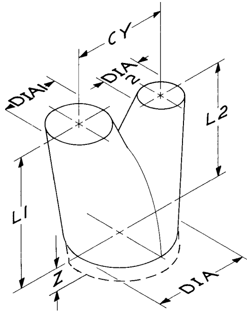
FIG. 38 Shape 7.1.6—Branch-Round-“Y”
