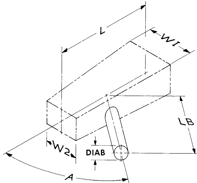
FIG. 37 Shape 7.1.5—Branch-Round-On Rectangular Reducer
