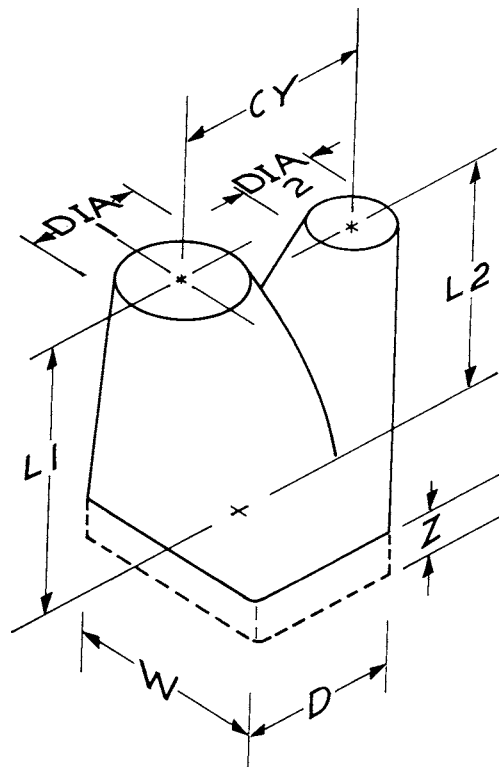
FIG. 39 Shape 7.1.7—Branch-Rectangular to Round “Y”
