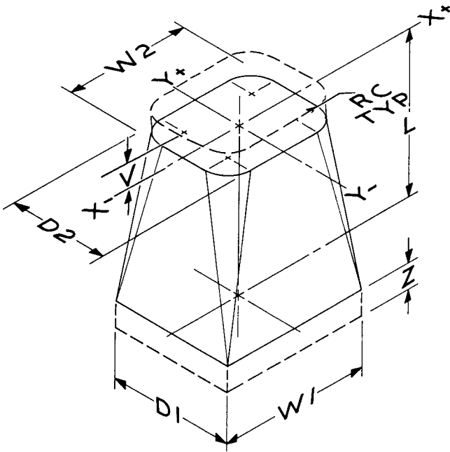
NOTE 1—Top or bottom, or both, of this shape may be slanted. FIG. 29 Shape 6.4—Transition-Rectangular to Radius Corner
