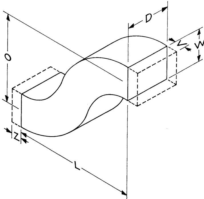
FIG. 9 Shape 2.4.1—Offset-Ogee-Without Splitters
