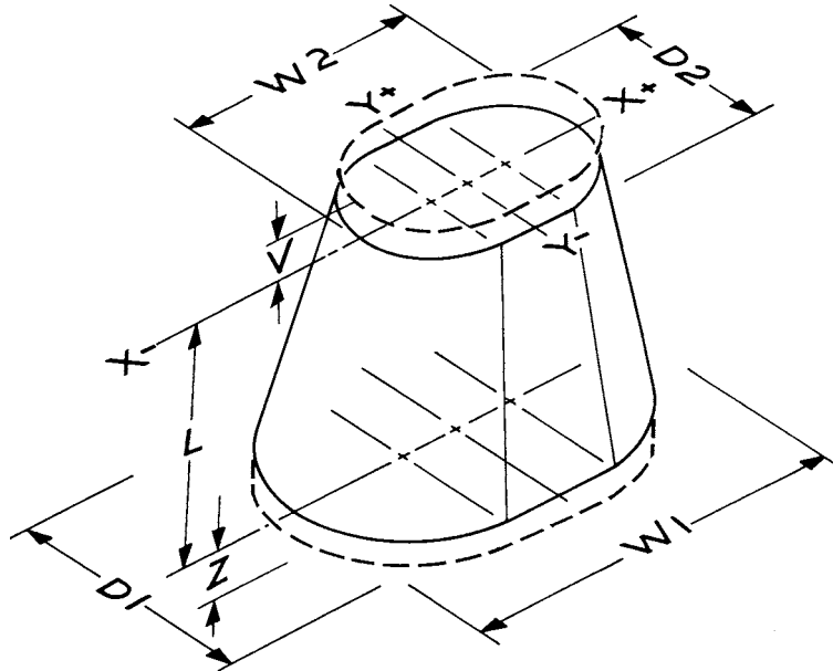
FIG. 24 Shape 5.2—Reducer-Flat Oval
