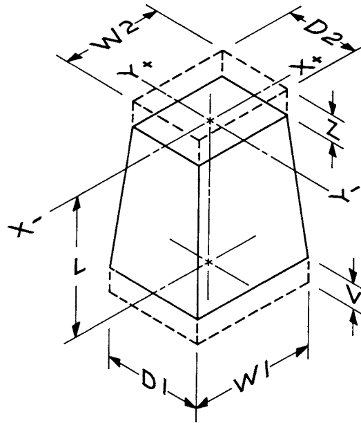
FIG. 25 Shape 5.3—Reducer-Rectangular
