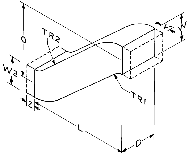
FIG. 11 Shape 2.5.1—Offset-Rectangular Reducing-Without Splitters
