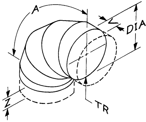
FIG. 13 Shape 3.1—Elbow-Round
