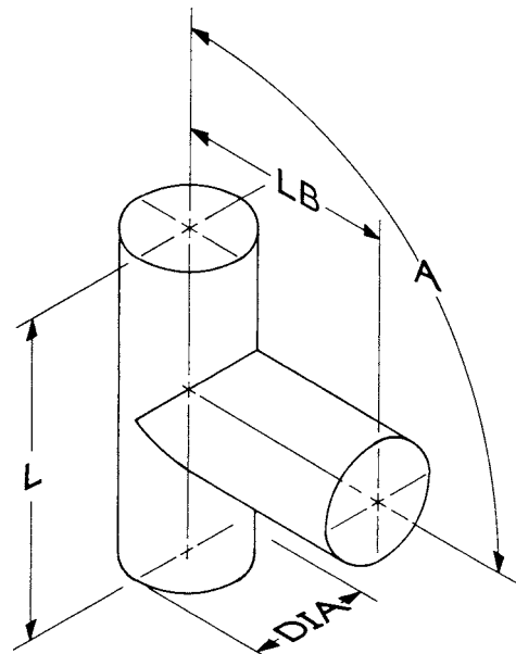
FIG. 33 Shape 7.1.1—Branch-Round-On Equal Diameter Round
