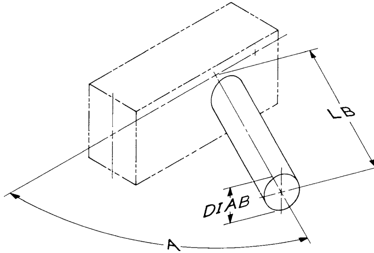
FIG. 36 Shape 7.1.4—Branch-Round-On Rectangular Straight
