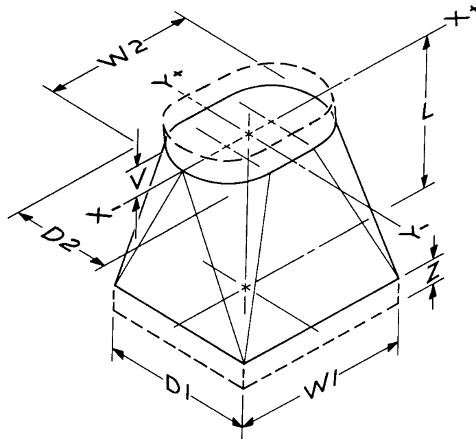
NOTE 1—Top or bottom, or both, of this shape may be slanted. FIG. 28 Shape 6.3—Transition-Rectangular to Flat Oval
