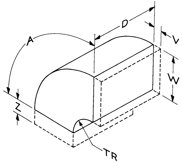
FIG. 16 Shape 3.3.1—Elbow-Rectangular-Without Splitters
