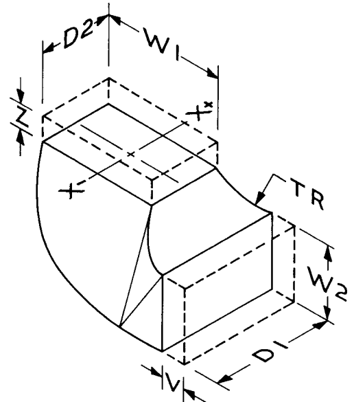
FIG. 20 Shape 3.5.1—Elbow-Rectangular Transition-Without Splitters
