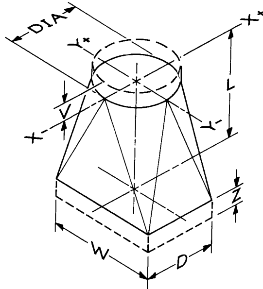
NOTE 1—Top or bottom, or both, of this shape may be slanted. FIG. 27 Shape 6.2—Transition-Rectangular to Round
