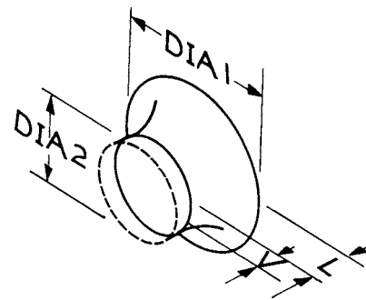
FIG. 31 Shape 6.6.1—Bellmouth-Round
