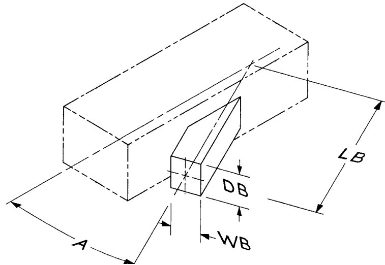
FIG. 40 Shape 7.2.1—Branch-Rectangular-On Rectangular Straight
