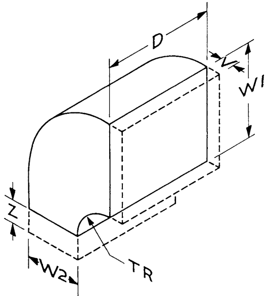
FIG. 18 Shape 3.4.1—Elbow-Rectangular Reducing-Without Splitters
