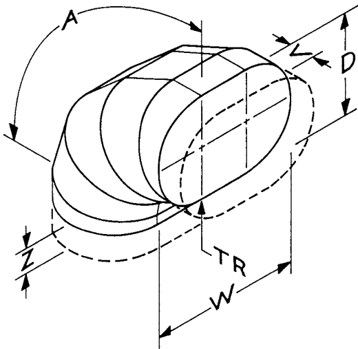
FIG. 15 Shape 3.2.2—Elbow-Flat Oval-Short Axis
