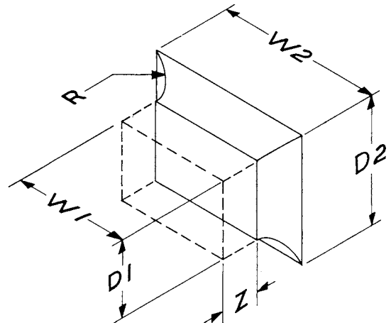
FIG. 32 Shape 6.6.2—Bellmouth-Rectangular
