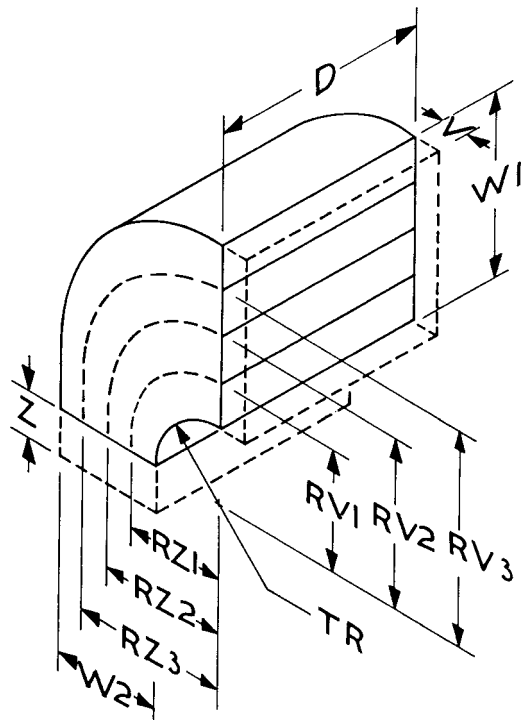
FIG. 19 Shape 3.4.2—Elbow-Rectangular Reducing-With Splitters
