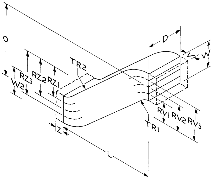
FIG. 12 Shape 2.5.2—Offset-Rectangular Reducing-With Splitters
