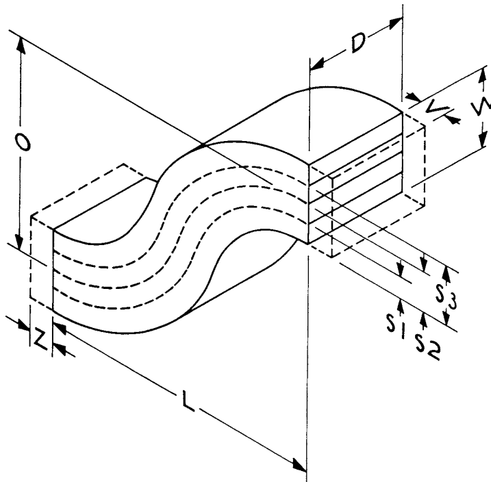
FIG. 10 Shape 2.4.2—Offset-Ogee With Splitters
