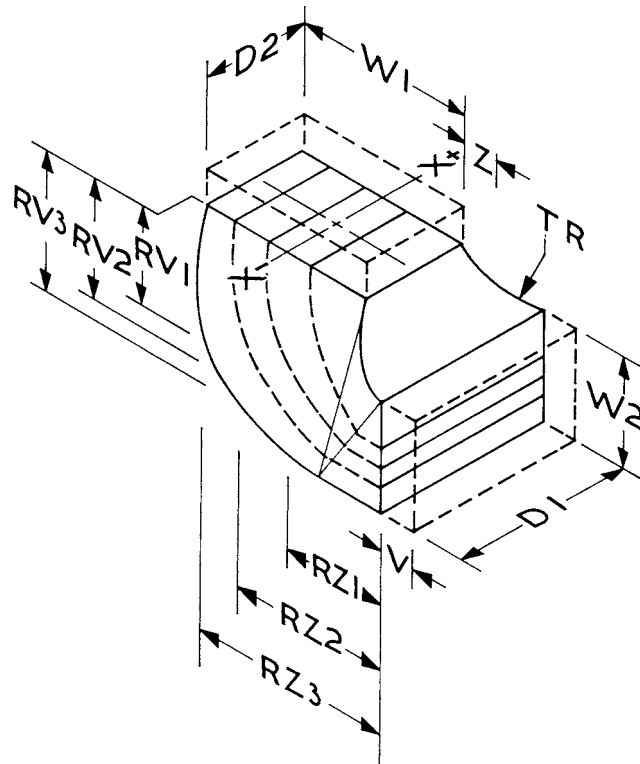
FIG. 21 Shape 3.5.2—Elbow-Rectangular Transition-With Splitters
