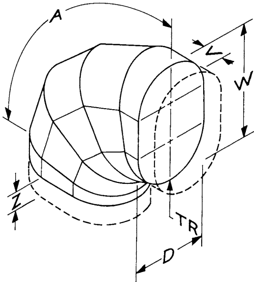
FIG. 14 Shape 3.2.1—Elbow-Flat Oval-Long Axis
