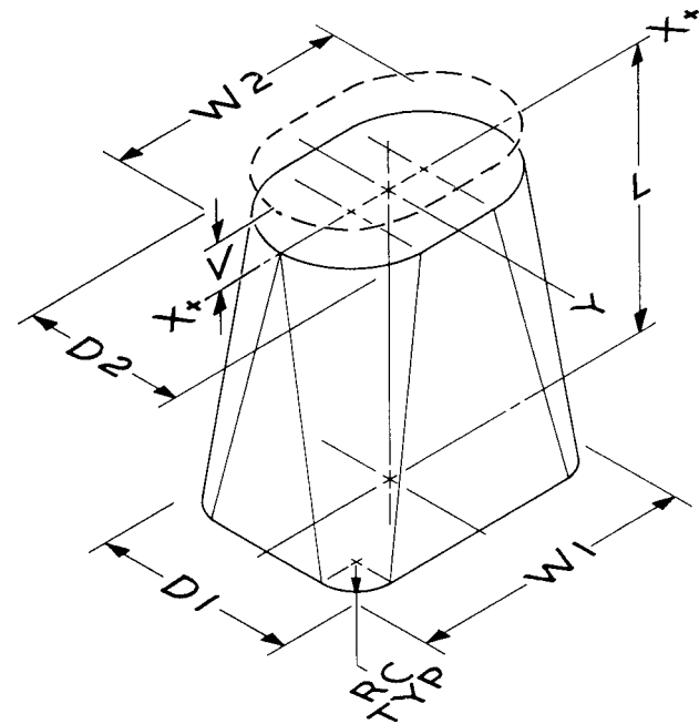
NOTE 1—Top or bottom, or both, of this shape may be slanted. FIG. 30 Shape 6.5—Transition-Radius Corner to Flat Oval
