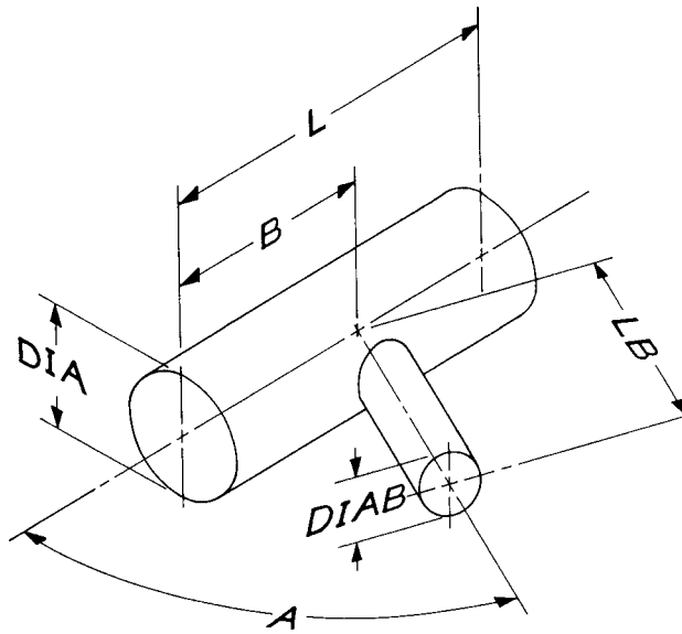
FIG. 34 Shape 7.1.2—Branch-Round-On Larger Diameter Round
