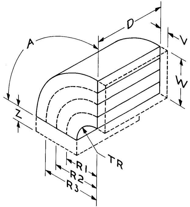
FIG. 17 Shape 3.3.2—Elbow-Rectangular-With Splitters
