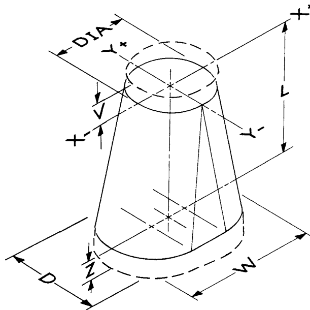
FIG. 26 Shape 6.1—Transition-Flat Oval to Round
