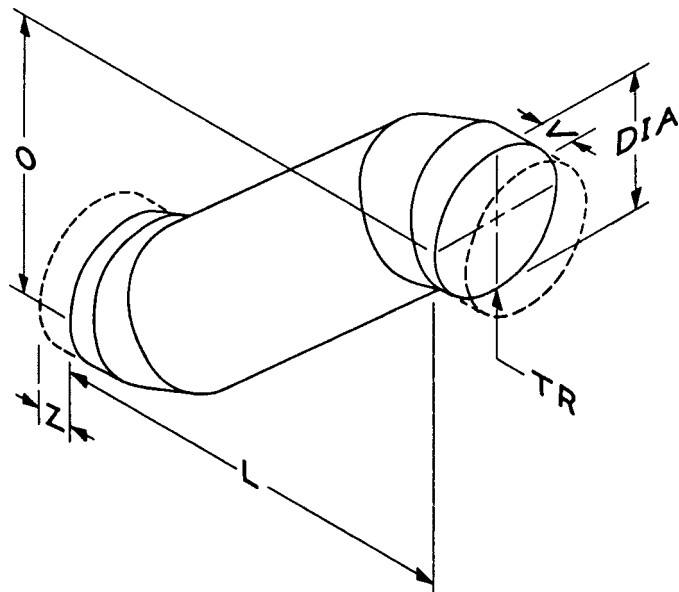
FIG. 4 Shape 2.1—Offset-Round
