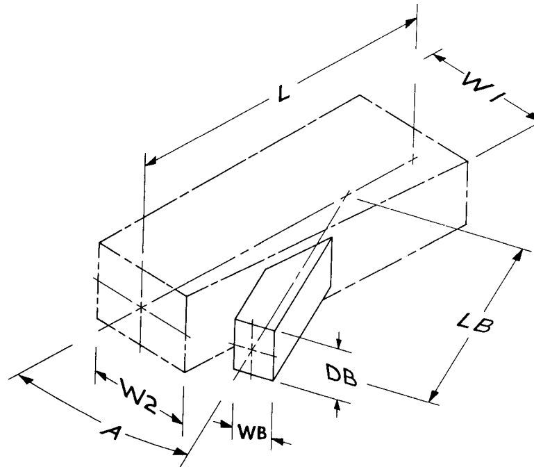
FIG. 41 Shape 7.2.2—Branch-Rectangular-On Rectangular Reducer
