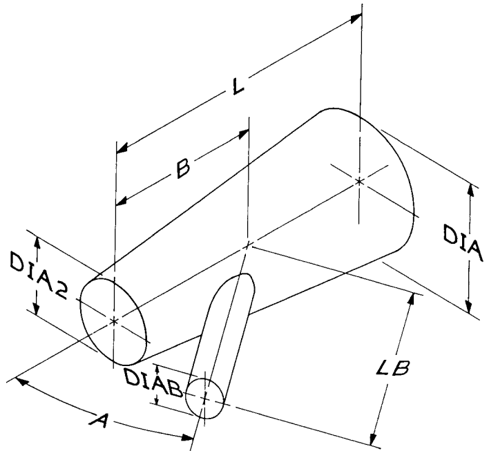
FIG. 35 Shape 7.1.3—Branch-Round-On Round Reducer
