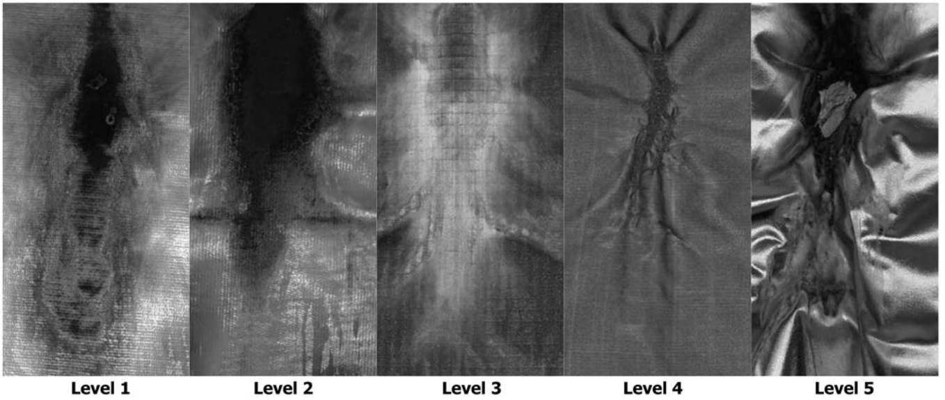
FIG. A1.3 Rating Photos for Shrinkage
