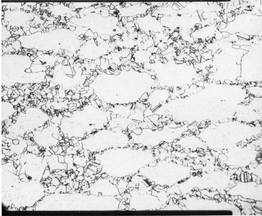
FIG. A1.4 100x, Necklace Condition Not Rateable to E930
