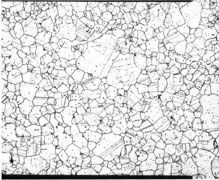
FIG. A1.2 50x, Wide-Range Condition Not Rateable to E930
