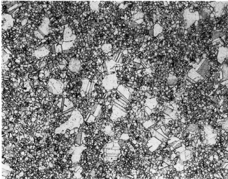
FIG. A1.3 100x, Bimodal Condition Not Rateable to E930
