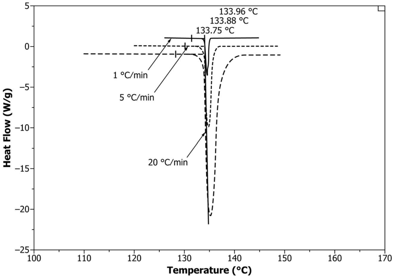
FIG. X1.1 Temperature Shift for Samples that Melt
