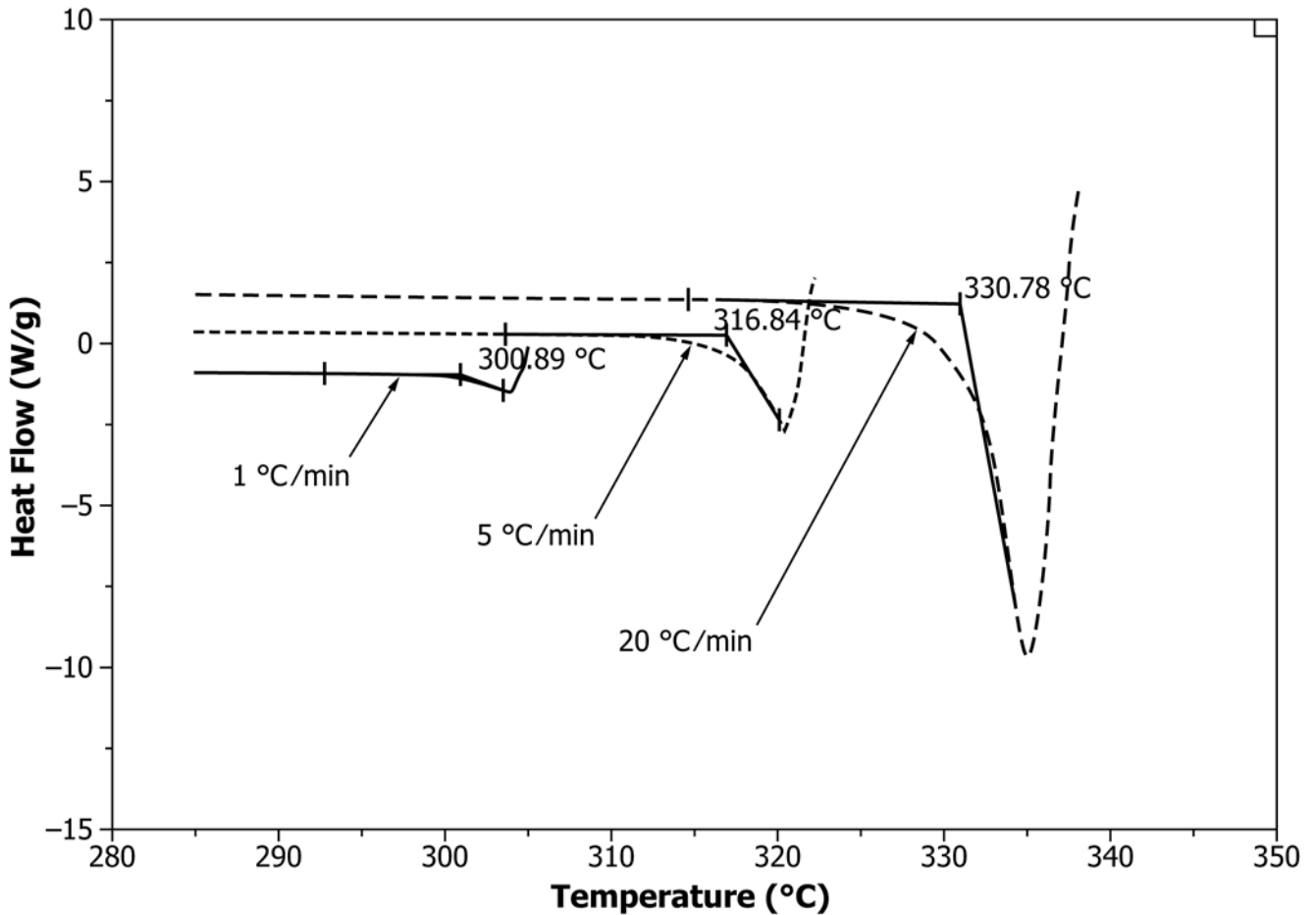
FIG. X1.2 Temperature Shift for Samples that Decompose
