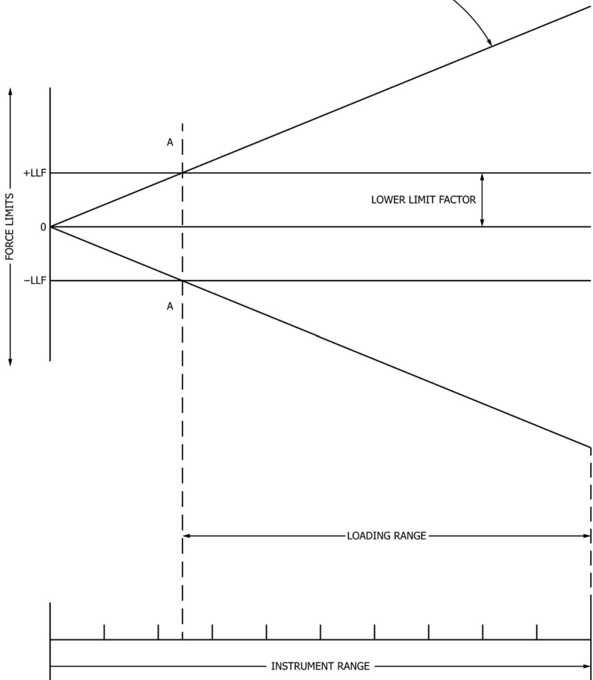
FIG. 1 Relationship of Loading Range to Instrument Lower Force Limit and Specified Limits of Error
