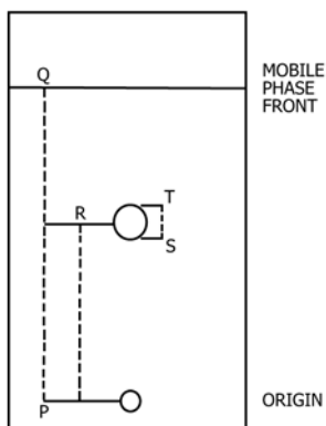
FIG. 2 Typical Planar Chromatogram
