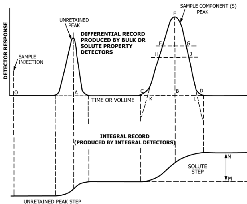
FIG. 1 Typical Chromatogram
