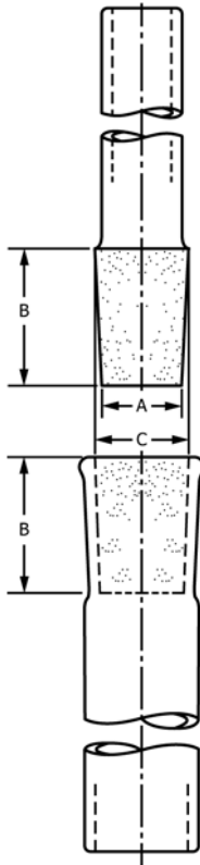
FIG. 1 Taper-Ground Joint
