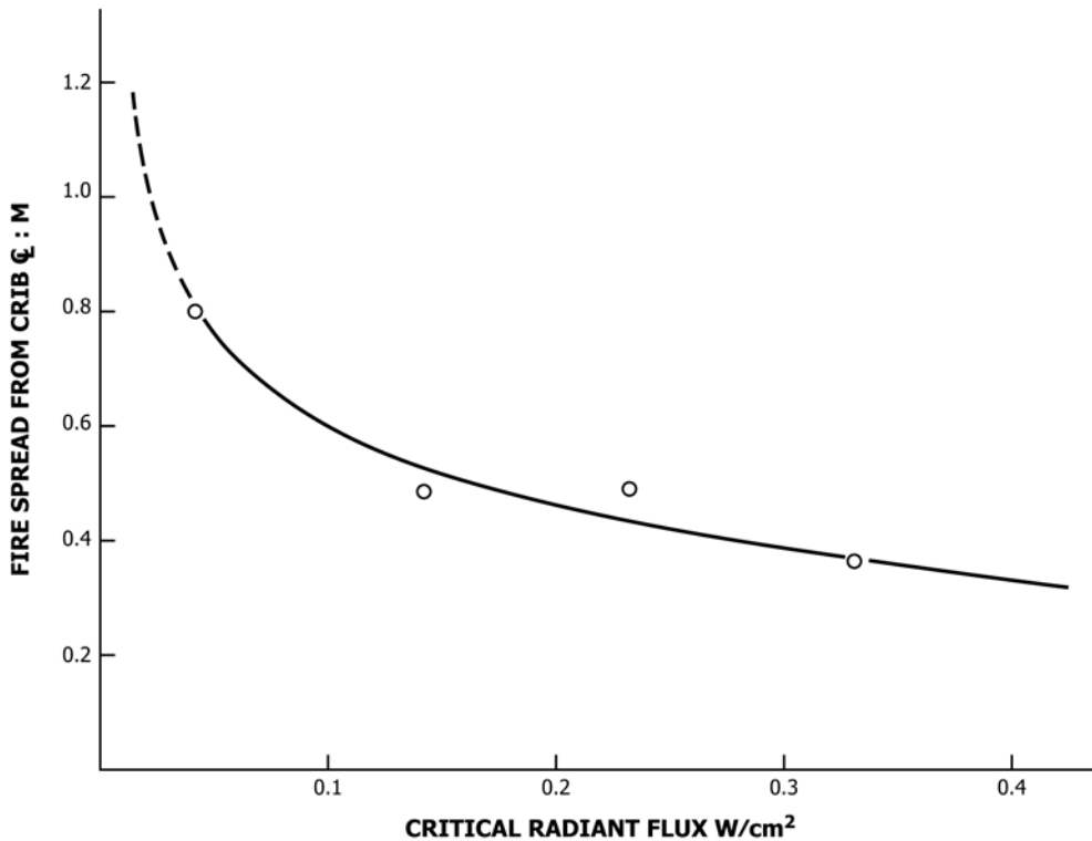
FIG. X1.2 Room Burn Tests—Fire Spread from Crib 6.4-kg Cribs
