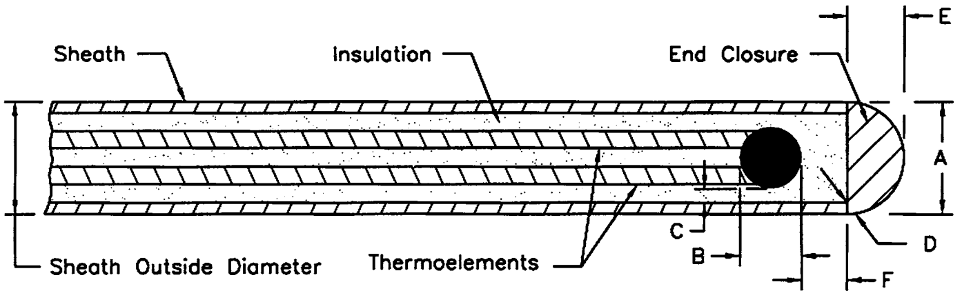
FIG. 1 Grounded Measuring Junction, Style G
