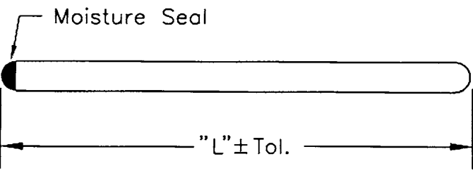
FIG. 3 Sheathed Thermocouple
