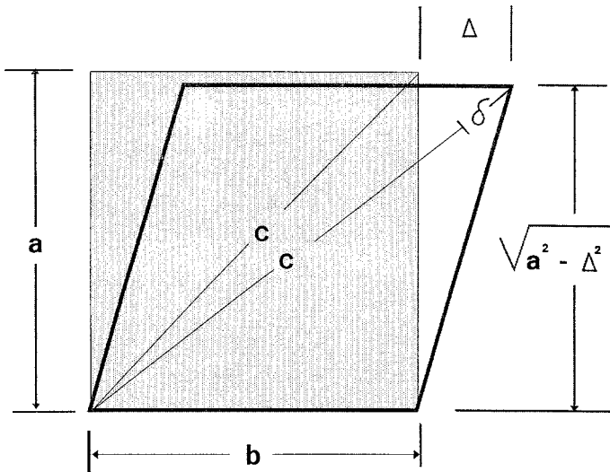
NOTE 1—Horizontal shear displacement calculated on the basis of the diagonal elongation simplifies the test by eliminating the need to measure rigid body rotation and horizontal translation of the wall.
