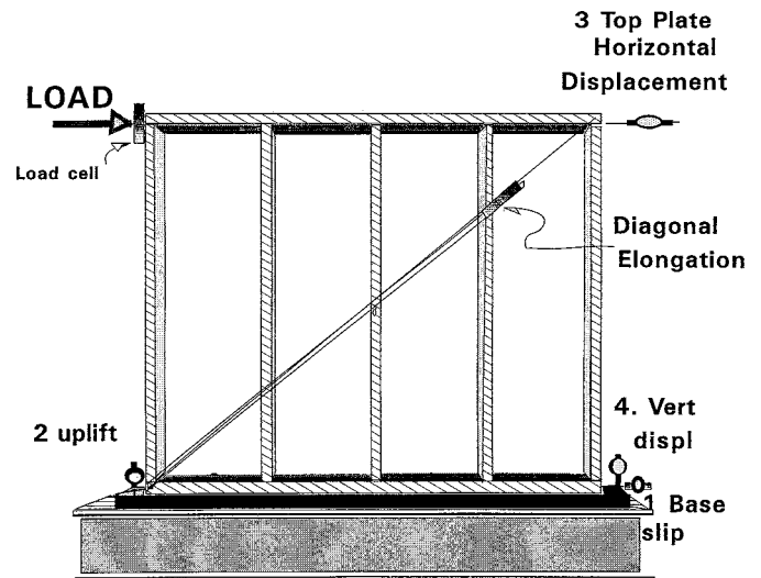
NOTE 1—The horizontal load is measured using a load cell in series with the loading ram. Wall shear displacement is determined using either four gages to separate shear from uplift, rotation, and horizontal slip of the wall or by measuring diagonal elongation to measure wall racking deformation directly. To restrain rigid-body rotation, apply boundary conditions to simulate those that control wall performance in service.
