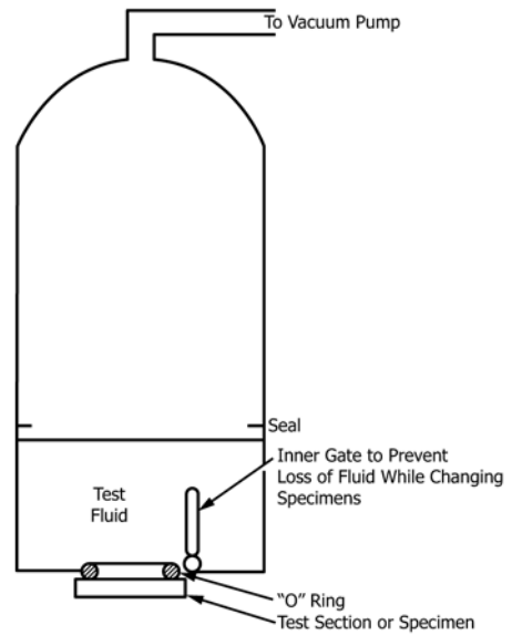
FIG. 1 Vacuum Chamber Technique
