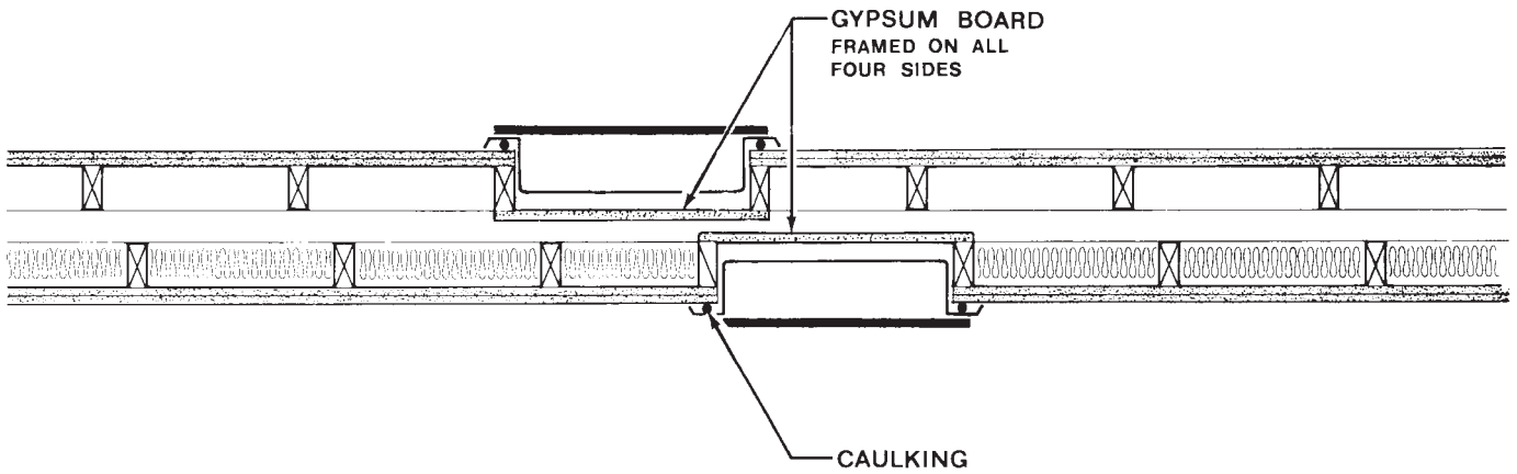
FIG. 16 Nearly Back-to-Back Cabinets Need Caulking and Backing with Gypsumboard
