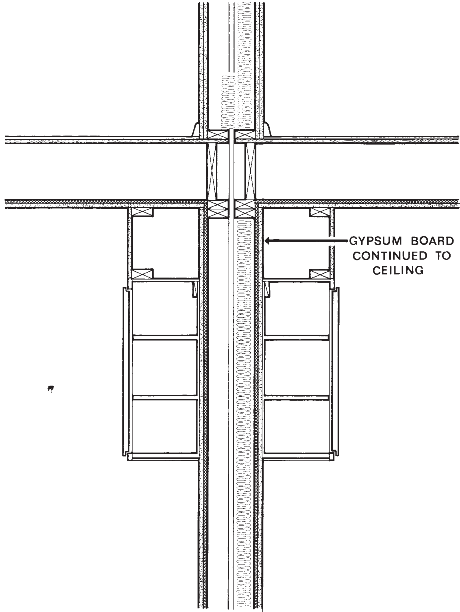
FIG. 10 Recommended Gypsum Board Application in Soffit Areas
