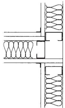
FIG. 12 (a) Recommended Gypsum Board Staggering at Corners
