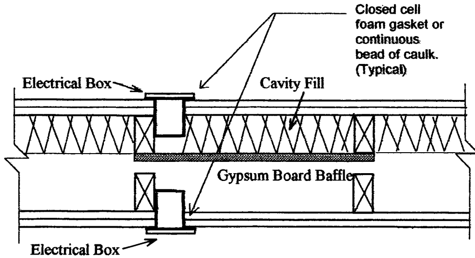
FIG. 14 Gypsum Board Baffles can be Used Where the Minimum Offset and Airtight Boxes can not be Utilized. The Baffle Should Extend at Least 24 in. (600 mm) Above and Below the Boxes and the Wall Cavity must Contain Insulation
