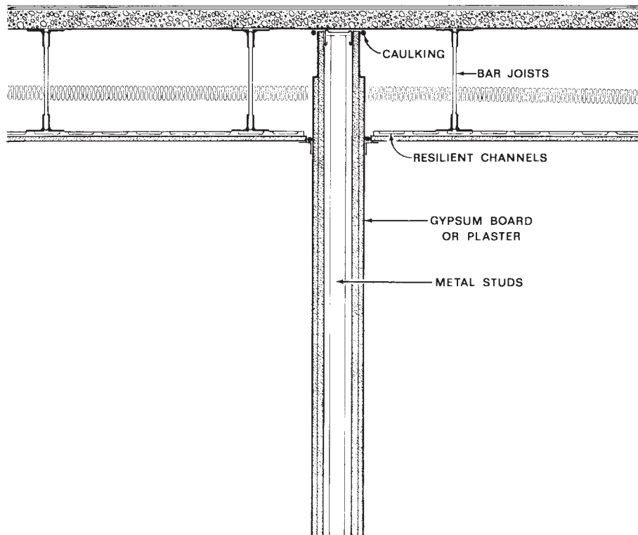
FIG. 7 A Partition Extended into an Open Ceiling to Prevent Flanking
