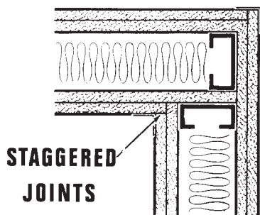
FIG. 12 (a) Recommended Gypsum Board Staggering at Corners
