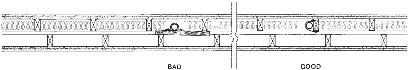
NOTE 1—Can cause a short circuit. When plumbing must be blocked, it is good practice to attach directly to the stud. FIG. 20 Coupling of Double Walls
