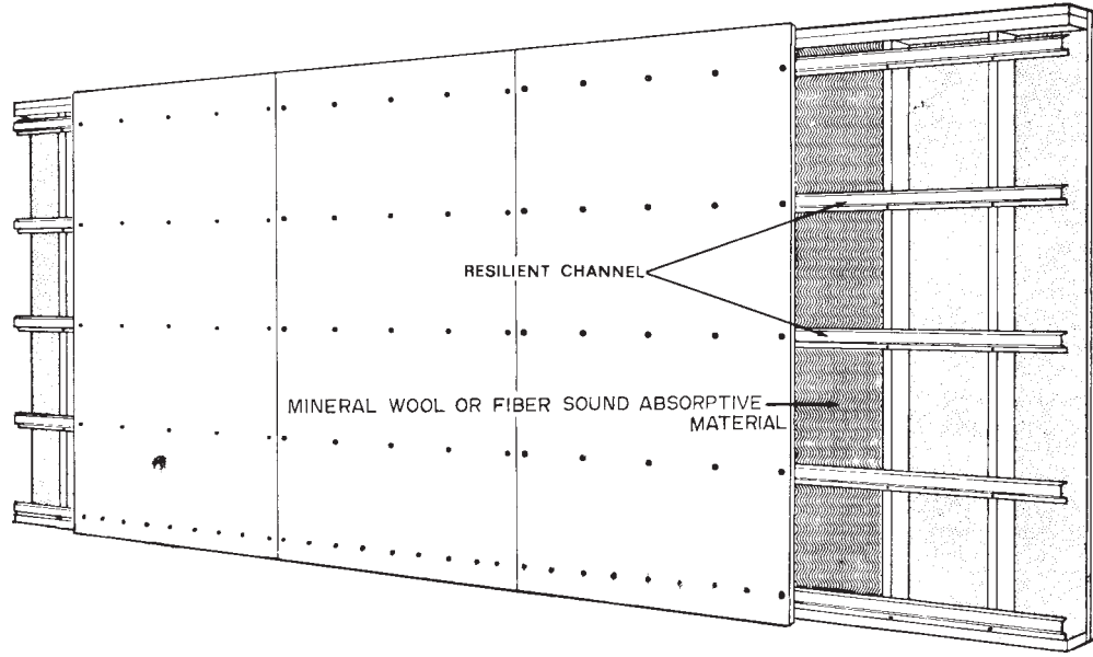
FIG. 19 An Example of Unequal Thicknesses of Surface Layers and Dissimilar Attachments
