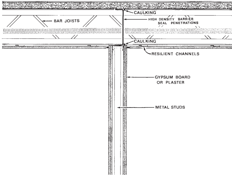
FIG. 6 A Barrier Recommended for Open Joist Ceiling Plenum
