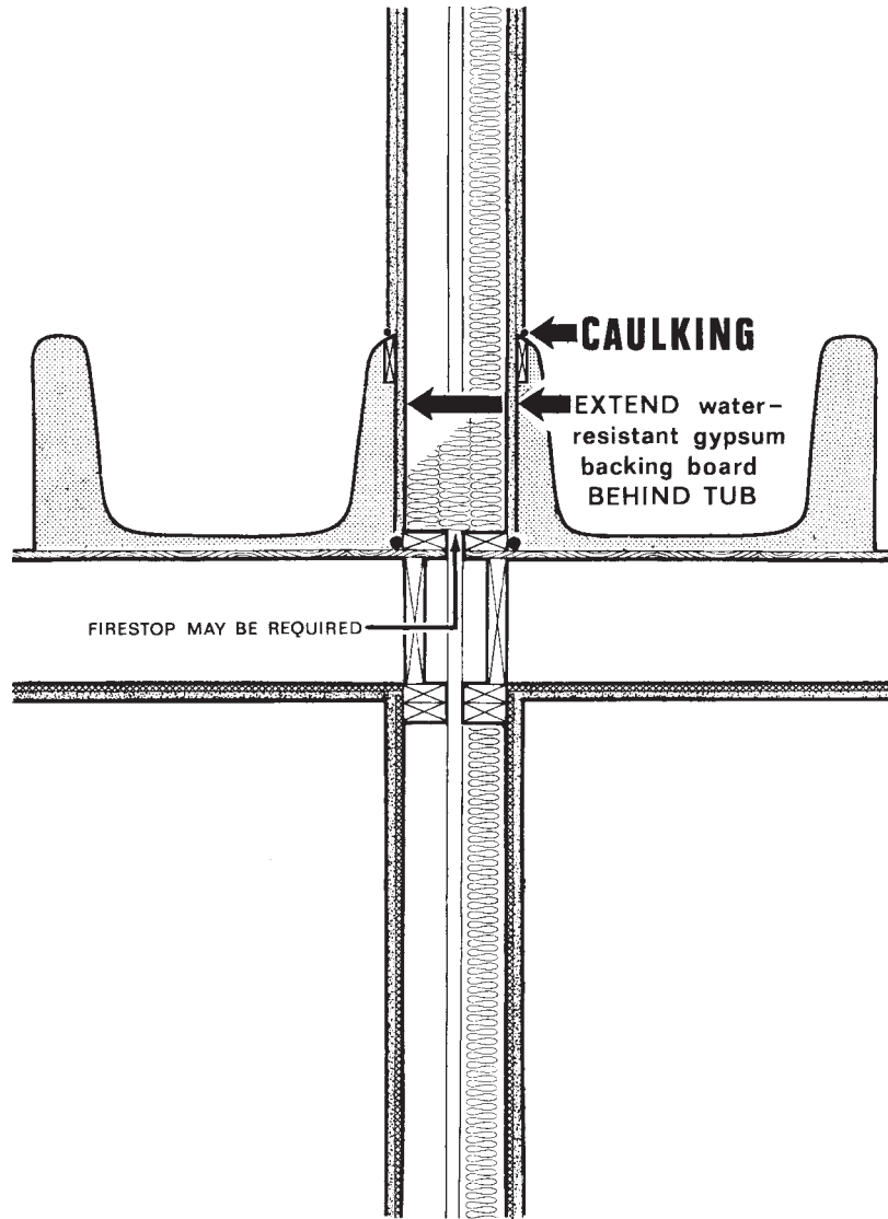
FIG. 9 Recommended Gypsum Board Application Behind Bathtubs
