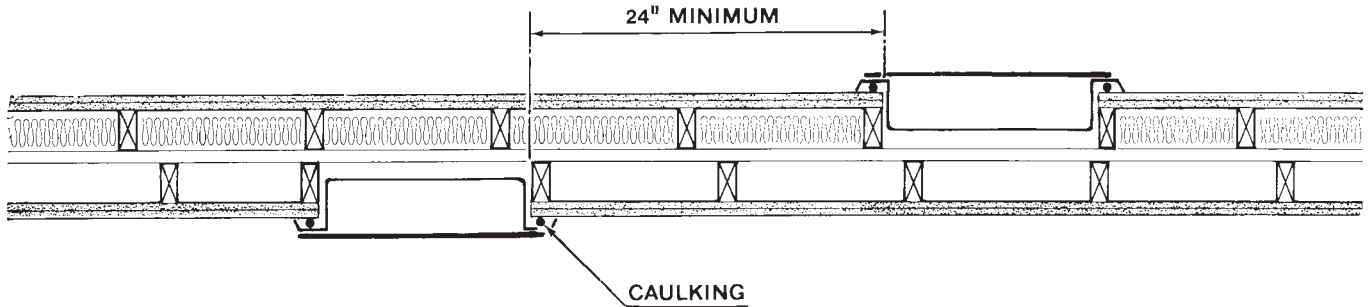
FIG. 15 Properly Spaced Cabinets Reduce Sound Transmission
