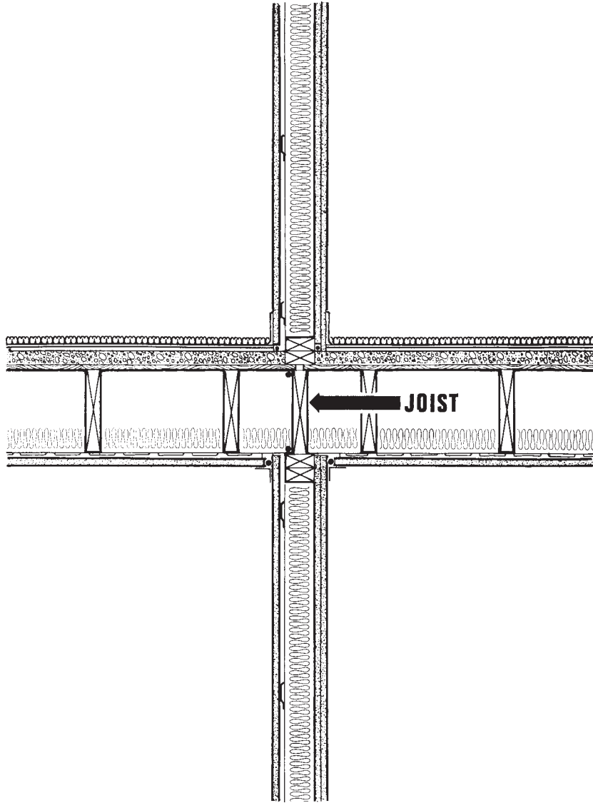
FIG. 8 A Single Parallel Joist Serves as a Flanking Barrier
