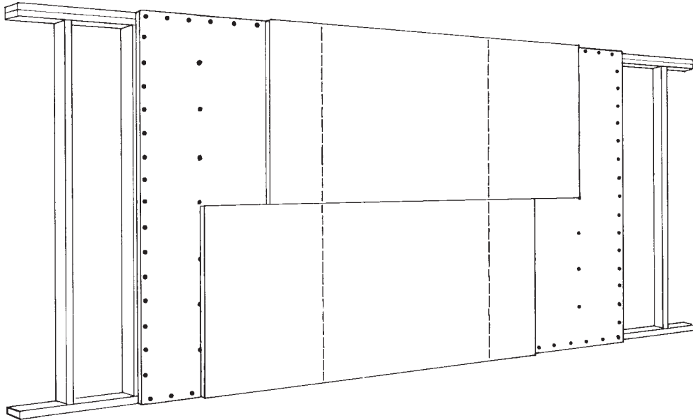
FIG. 18 A Recommended Arrangement of Multiple Layer of Gypsum Board
