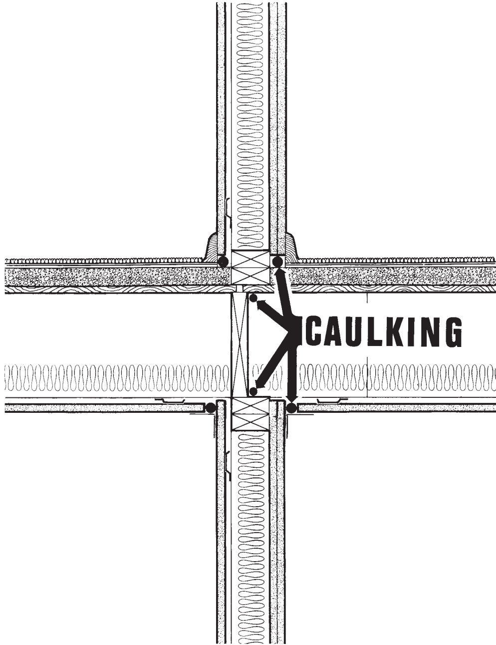
FIG. 11 Caulking to Prevent Possible Sound Leaks
