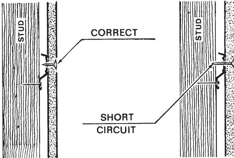
FIG. 17 Vibration Isolation Obtained with Resilient Channels is Lost if Screws are Too Long
