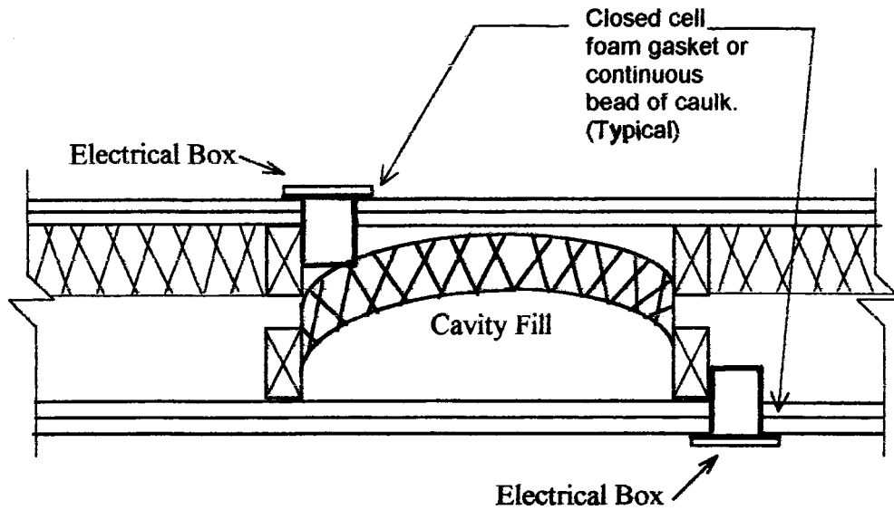
FIG. 13 Offset Electrical Boxes (600 mm or 24 in.) Showing the Preferred Method of Installing the Cavity Insulation so that the Backs of the Boxes are Covered
