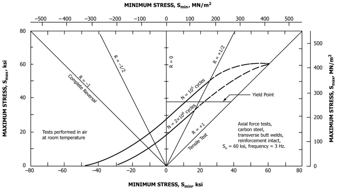
MINIMUM STRESS, S_{min} , ksi FIG. 2 Constant-Life Diagram
