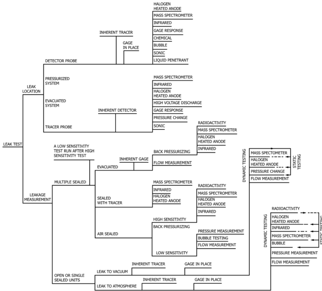
FIG. 1 Guide for Selection of Leakage Testing Method
