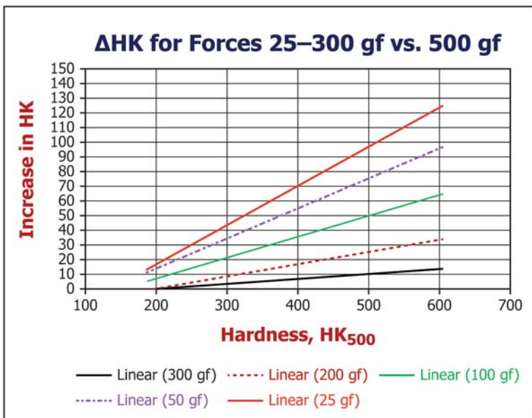
FIG. X5.18 Graph based upon the data shown in X5.17 showing the increase in HK compared to the HK 500 value for test forces 25, 50, 100, 200 and 300 gf. These values would be subtracted from the HK value at test loads from 25 to 300 gf to approximate the HK 500 value.
