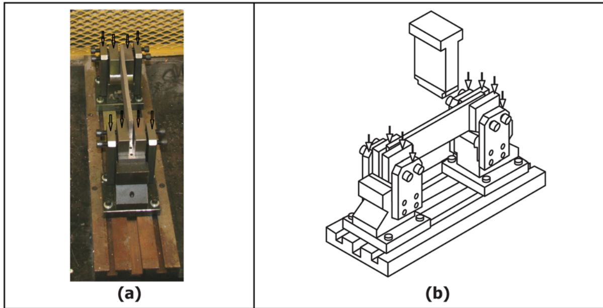
FIG. 3 An example of optional anti-buckling guides for pipe steel specimens with wall thickness less than 10 mm
