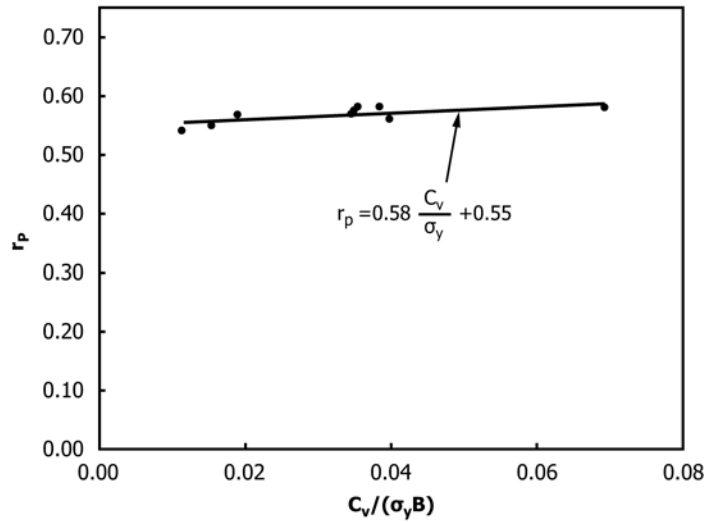
FIG. 6 Rotation factor versus C_v/(\sigma_y B) for impact test results
