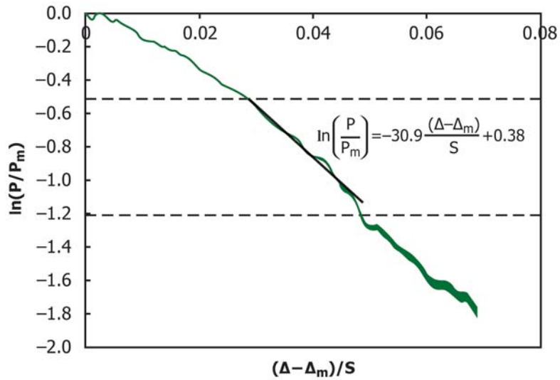
FIG. 5 Plot of \ln(P/P_m) versus (\Delta-\Delta_m)/S for all data points beyond the maximum force point ( P_m, \Delta_m ), illustrating the determination of the slope for CTOA_{B/2} . In this example, \xi = 30.9 .
