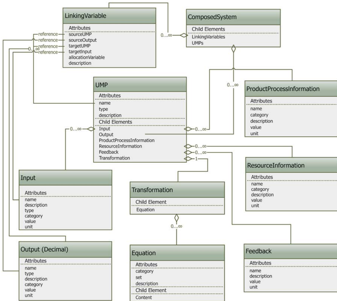
FIG. 5 UML Representation Showing Relations between Elements in UMP Information Structure
