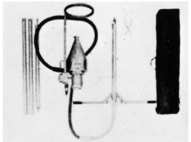
FIG. 15 Vacuum Sampler
