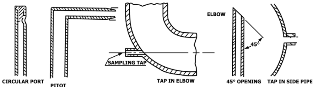
FIG. 23 Sampling Probes and Taps
