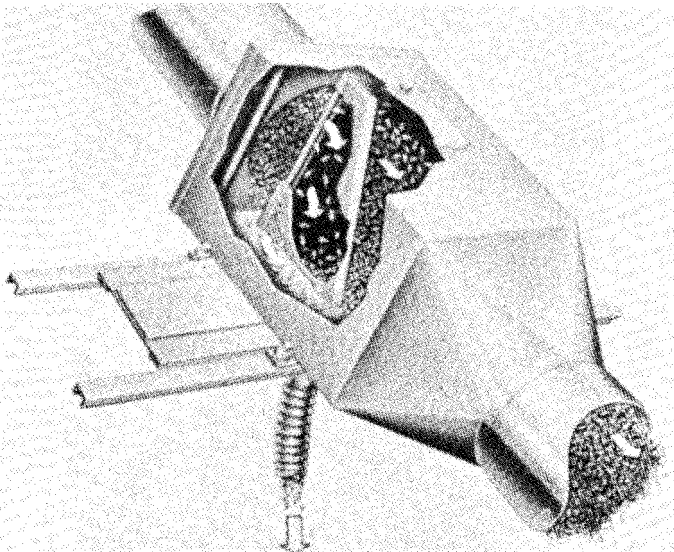
FIG. 18 Cross-Cut Sampler
