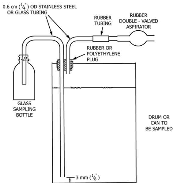
FIG. 7 Alternative Tube Sampling Assembly
