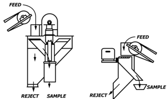
FIG. 17 Falling-Stream Samplers
