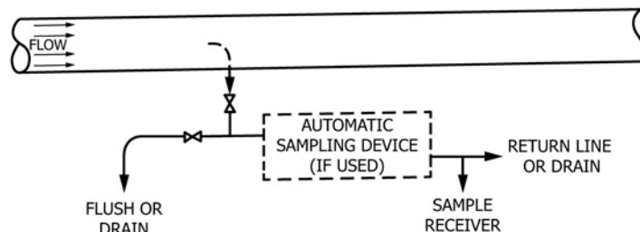
(D) TYPICAL ASSEMBLY FOR CONTINUOUS SAMPLING
