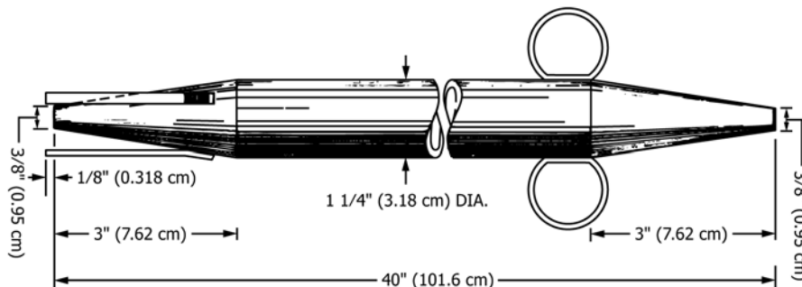
FIG. 6 Sampling Tube
