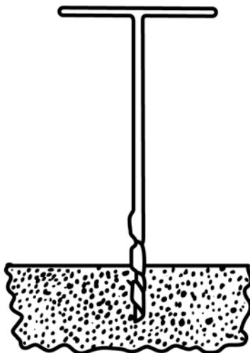
FIG. 14 Auger Sampler
