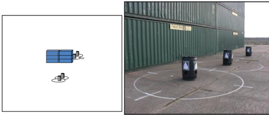
Left: The non-line-of-sight range test method uses an airstrip or flat, paved road with robot test stations placed in front of and behind a wall constructed of stacked 12 m (40 ft) International Standards Organization (ISO) shipping containers. Right: Robot test stations are prototyped behind the wall with targets on the barrels for visual inspection tasks and circular paths for maneuvering tasks.
