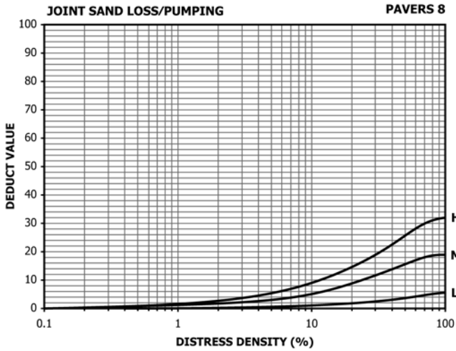
FIG. X3.8 Joint Sand Loss/Pumping
