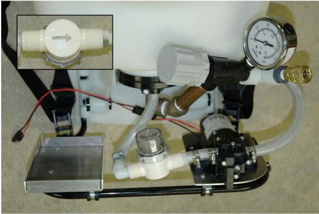
FIG. A1.4 Mount Pump
