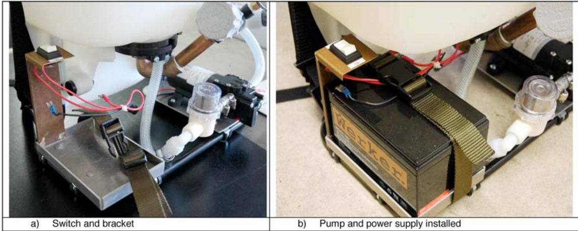
FIG. A1.5 Power Supply Installation
