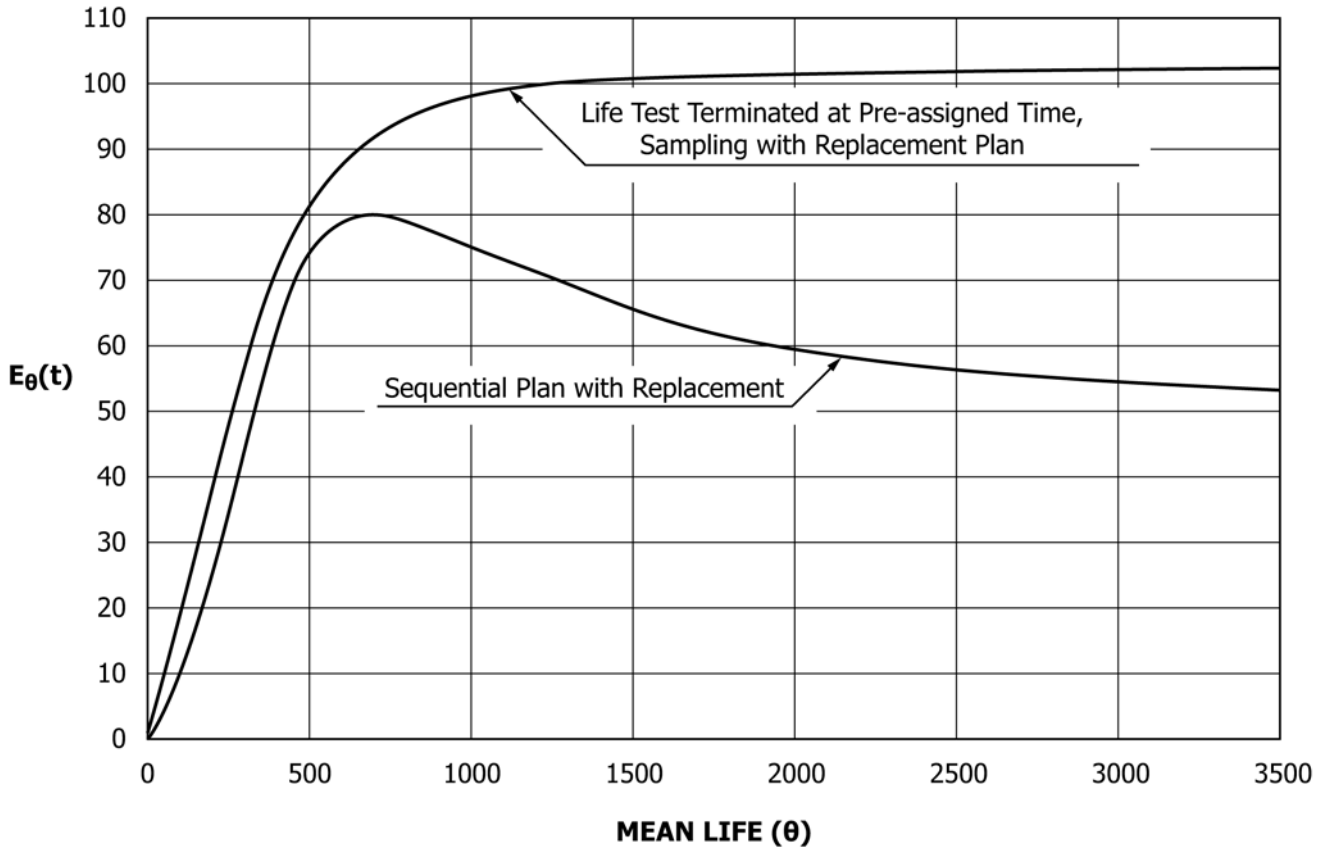
FIG. A1.5 Comparison of Expected Waiting Time Required for Decision for Sequential and Life Test Terminated at Preassigned Time, Sampling With Replacement Plans
