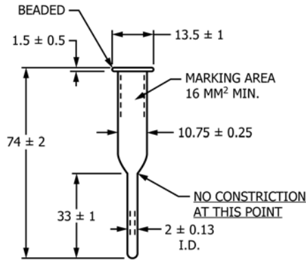
FIG. 4 Centrifuge Tube, Conical Bottom, Stoppered and Graduated
