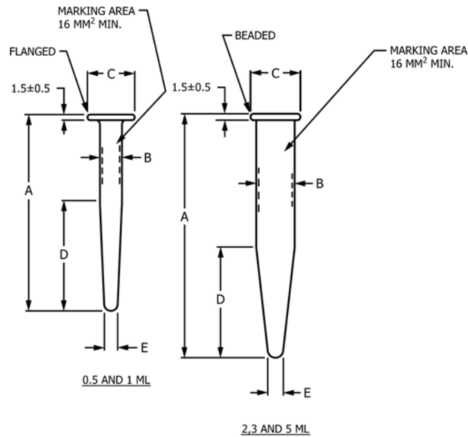
FIG. 2 Centrifuge Tubes, Conical Bottom, Plain (see Table 2)
