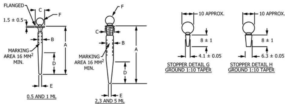
FIG. 2 Centrifuge Tubes, Conical Bottom, Plain (see Table 2)
