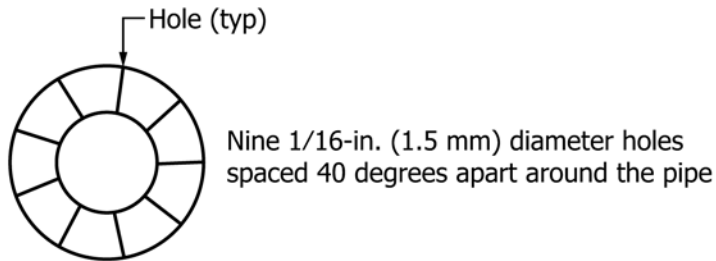
Enlarged Section View A - A
