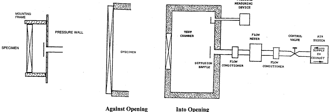
FIG. 1 General Arrangement of the Air Leakage Apparatus
