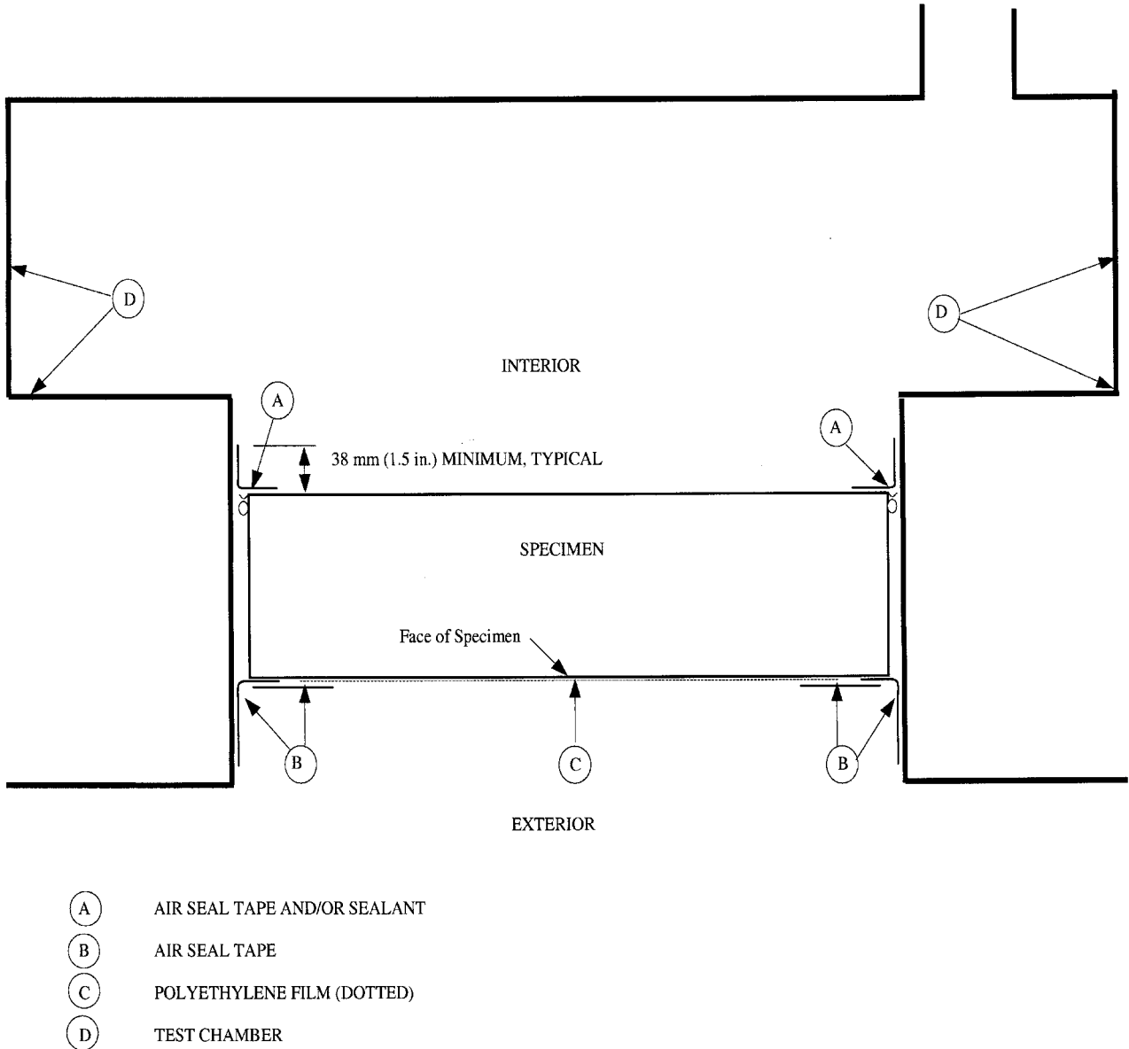
FIG. 2 Arrangement of Air Leakage Apparatus with Specimen Fit into Test Chamber
