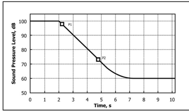
FIG. 1 Idealized Decay Curve and the Fitting Process
