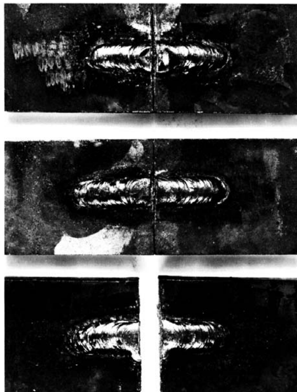
NOTE 1—The weld shown does not comply with the current procedure which specifies that the weld shall start from either end and shall proceed without interruption.
