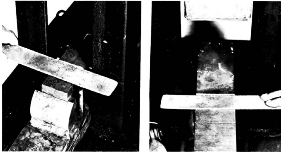
FIG. 12 Method for Alignment of Specimen
