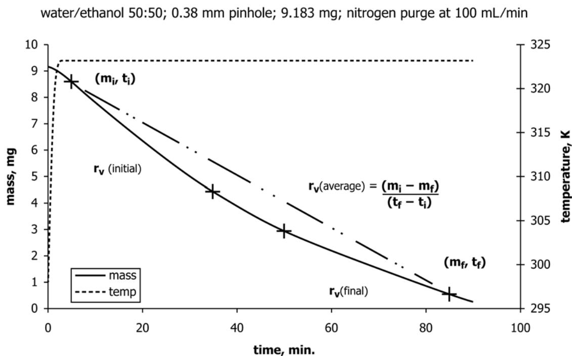
FIG. 3 Test Method A—Two Component Mixture
