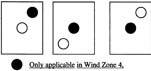
FIG. X4.1 Additional Large Missile Impact Locations in Wind Zone 4
