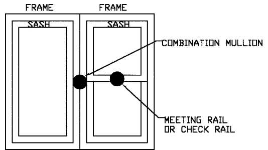
FIG. X4.3 Combination Mullion with Meeting or Check Rail
