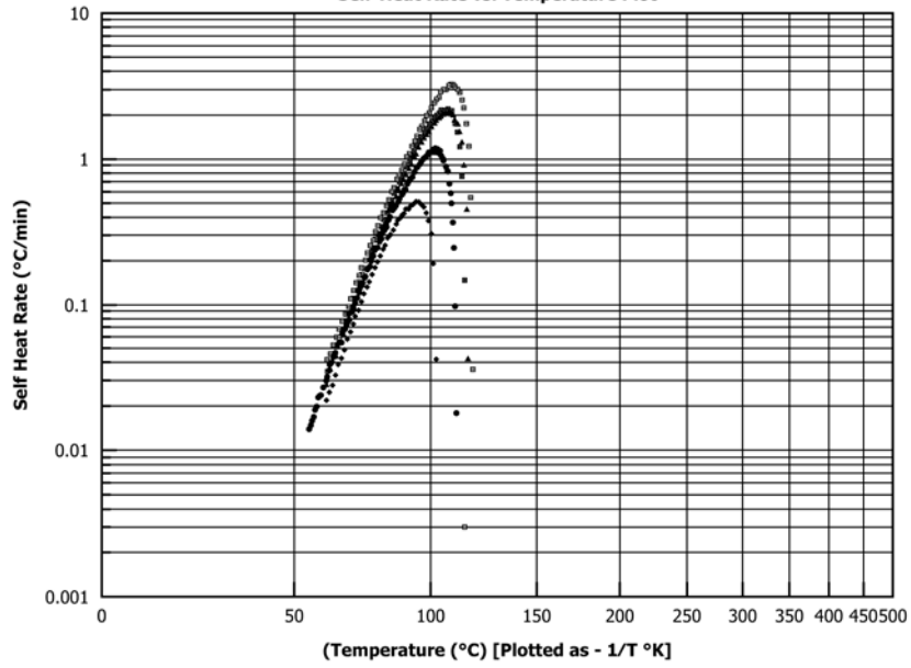
FIG. X1.2 2,2'-Azobisisobutyronitrile (12 Weight Percent in Dichloromethane) Self-Heat Rate versus Temperature Plot
