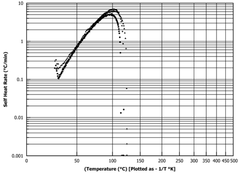
FIG. X1.3 2 to 1 Molar Ratio—Methanol to Acetic Anhydride Self-Heat Rate versus Temperature Plot
