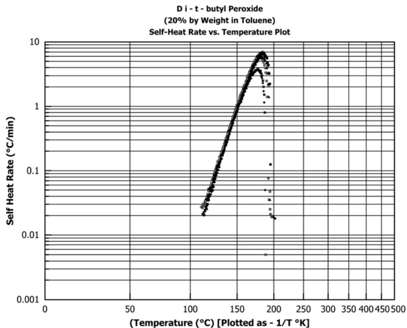
FIG. X1.1 Di-t-Butyl Peroxide (20 Weight Percent in Toluene) Self-Heat Rate versus Temperature Plot
