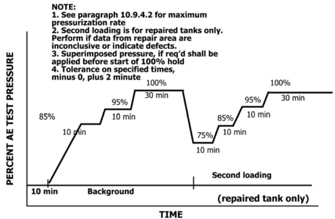
FIG. 3 In Service Tank Fill Schedule
