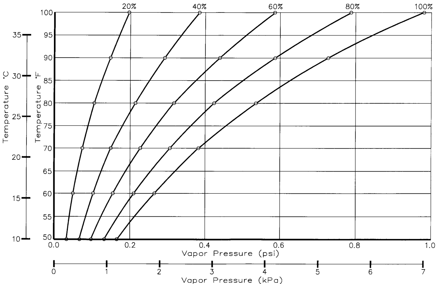
FIG. X1.1 Vapor Pressure of Moisture in Air at Different Temperatures and Relative Humidities. (Source: Ashok Kakade)
