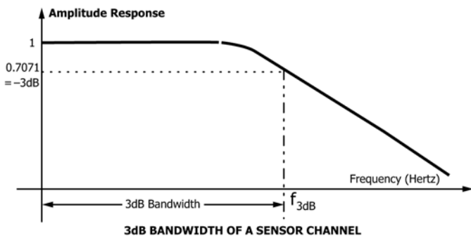
FIG. 2 Bandwidth
