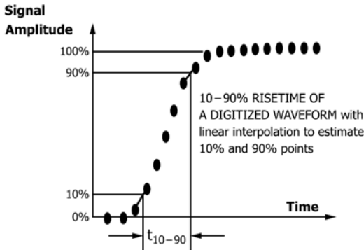
FIG. X2.2 Step Responses
