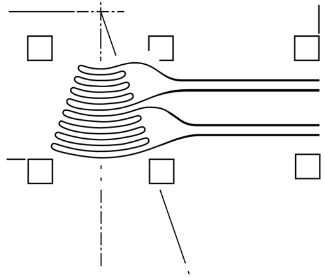
FIG. 6 Collinear-Focused EMAT Coils for Surface Wave Transduction
