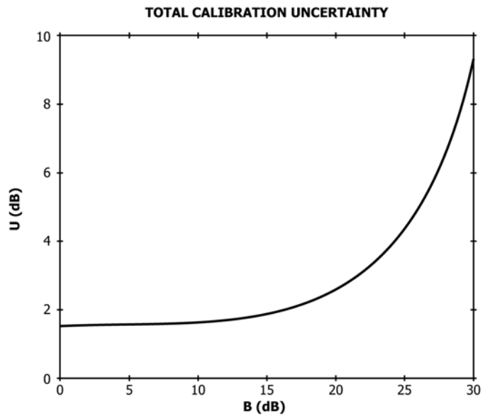
FIG. 8 Estimated Uncertainty, U , of the Calibration Frequency Response Data—Let M be the Largest Value of w_m over the Range 100 kHz to 1 MHz; Then, for any w_m , B = M - w_m , and the Uncertainty of w_m is \pm U
