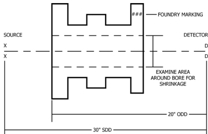
FIG. X1.2 Radioscopic Shooting Sketch
