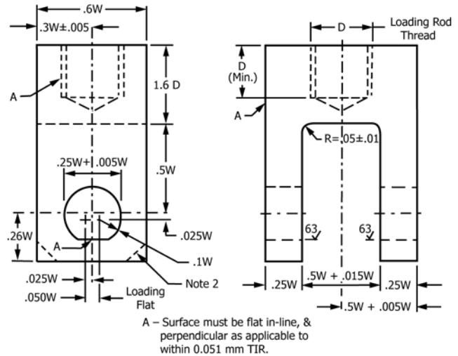
A – Surface must be flat in-line, & perpendicular as applicable to within 0.051 mm TIR. NOTE 1—Pin diameter = 0.24 W (+0.000W/–0.005W). For Specimens a with \sigma_{vs} > 1379 MPa the holes in the specimen and in the clevis may be 0.3W (+0.005W/–0.000W) and the pin diameter = 0.288W (+0.000W/–0.005W) NOTE 2—Corners of the clevis may be removed if necessary to accommodate a clip gage FIG. 2 Tension Test Clevis Design
