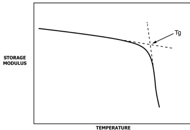
FIG. 1 Storage Modulus
