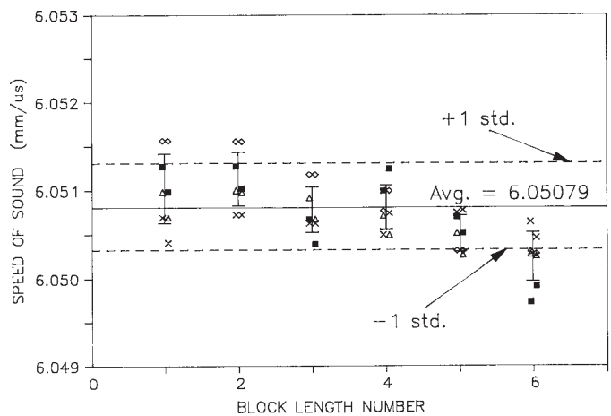
NOTE 1—Four different ultrasonic transducers were used and are indicated by different symbols. Two sets of values were taken for each transducer. "I" bars are estimated error limits for all the data of one path length as determined from the standard error deviation of each set. The average value and the standard deviation of the total data set are shown.
