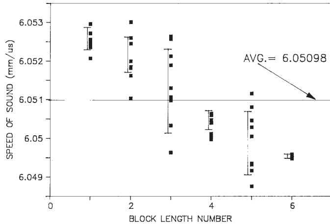
NOTE 1—The error “I” bars are determined from the average and the standard deviation of each path length set. The average is for the total set. FIG. X1.2 Generated Data Set to Demonstrate a Definite Failure to the Necessary Criterion of Speed of Sound = Constant
