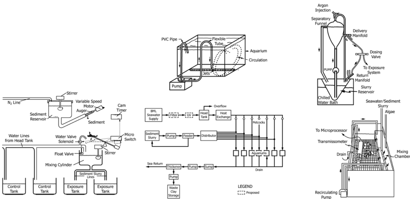
FIG. A1.2 Recirculating Tests
