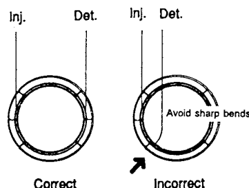
FIG. 10 Avoid Sharp Bends When Installing Fused Silica Capillary Column
