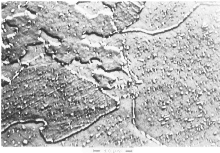
FIG. 5 Example of Replica Microstructure at 2000x SEM. Material: See Specification A335/A335M , Grade P22. Etchant: 2 % Nital
