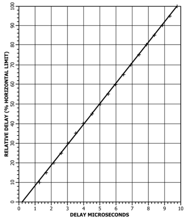
NOTE 1—Data points were taken by Method A using an actual instrument.
