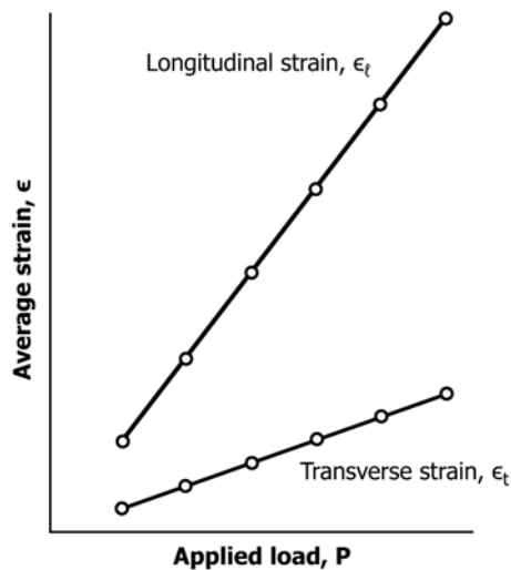
FIG. 2 Plot of Average Strains versus Applied Force for Determination of Poisson's Ratio
