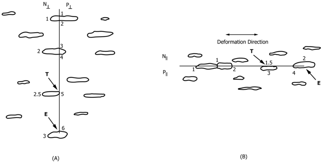
NOTE 1—The test grid lines have been shown oriented perpendicular (A) to the deformation axis and parallel (B) to the deformation axis. The counts for N_{\perp} , N_{\parallel} , P_{\perp} , and P_{\parallel} are shown for counts made from top to bottom (A) or from left to right (B). NOTE 2— T indicates a tangent hit and E indicates that the grid line ended within the particle; both situations are handled as shown.
