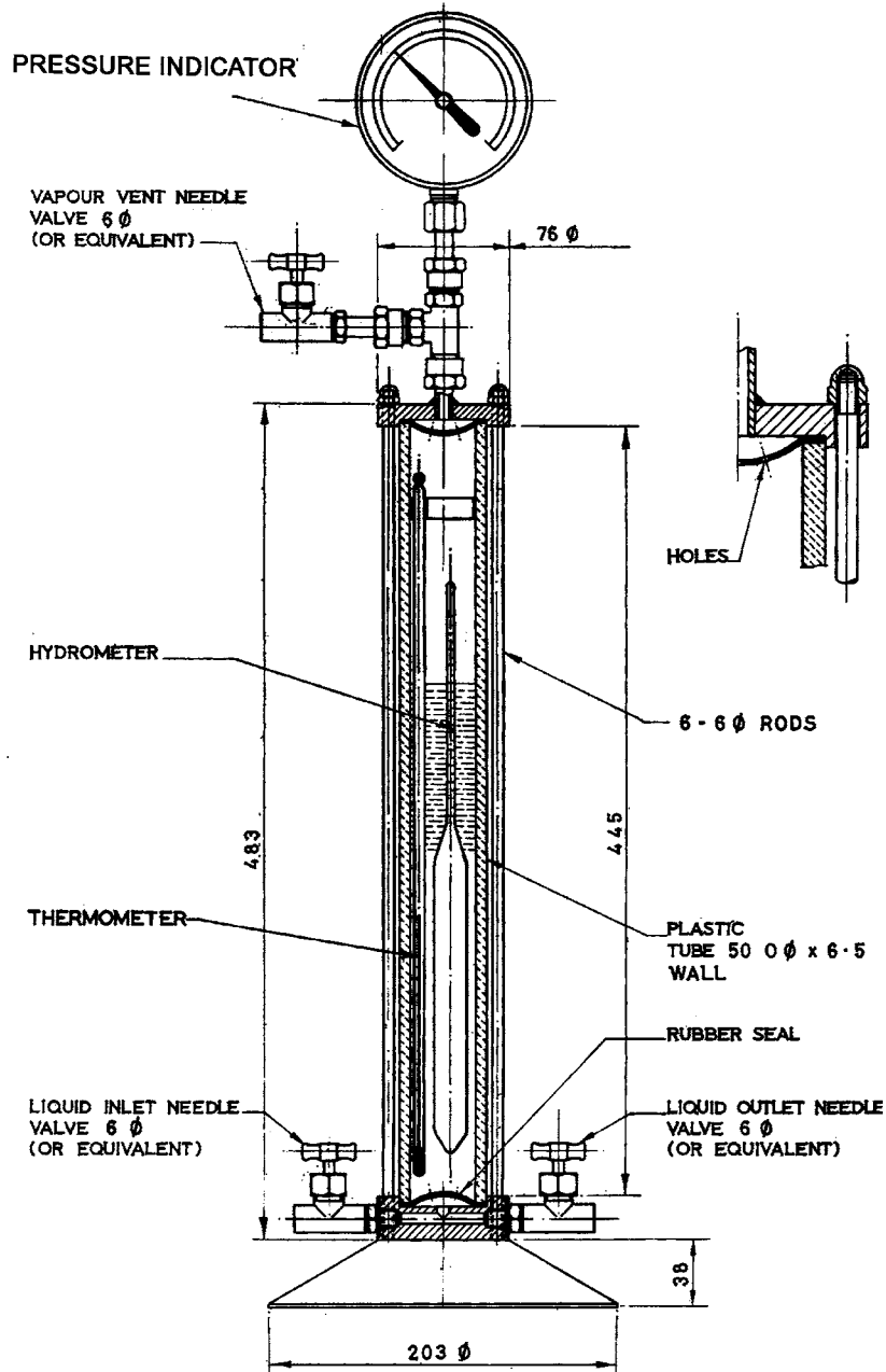
FIG. X1.1 Pressure Hydrometer Cylinder Comparator
