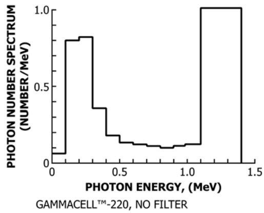
FIG. X1.8 Typical Spectrum for Shielded-Cavity Irradiator (4)
