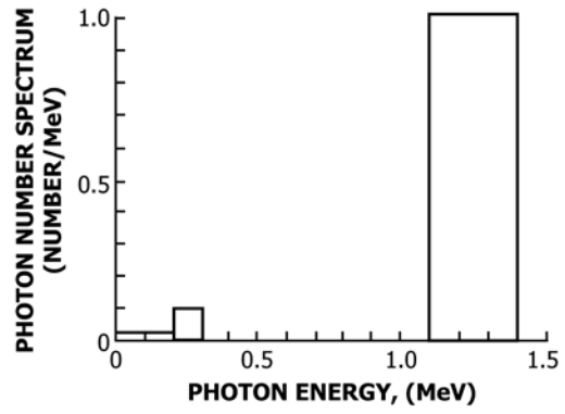
HDL CONCRETE ROOM, POS. A, .063" Pb
