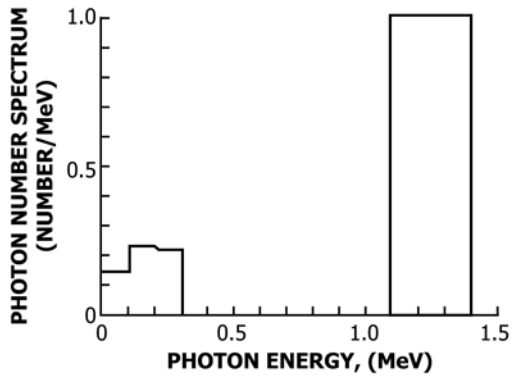
HDL CONCRETE ROOM, POS. A, NO FILTER
