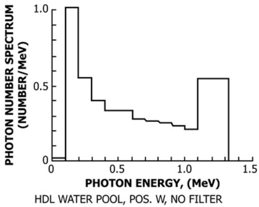
FIG. X1.6 Typical Spectra for Water Well Sources Under Various Conditions (4, 6)
