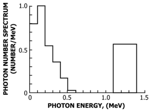
HDL CONCRETE ROOM, POS. B, NO FILTER
