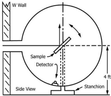
FIG. 2 Integrating Sphere (Reflectance Mode)
