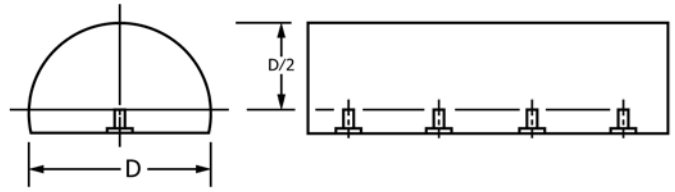
FIG. 2 Typical Area-Amplitude Reference Block for use in Ultrasonic Testing of Round Bars as in Fig. 1
