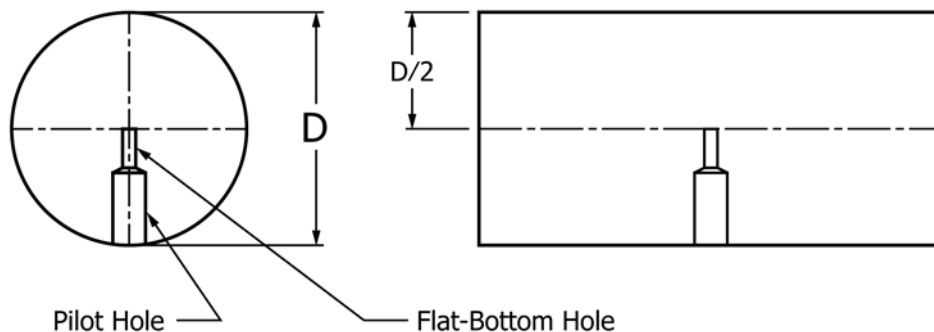
FIG. X1.1 Flat-Bottom Hole Placed at the Center of a Round Bar by This Method
